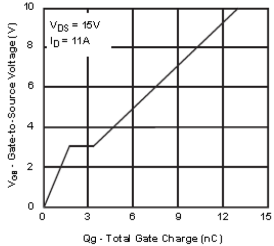
Fig. 8 Gate Charge
